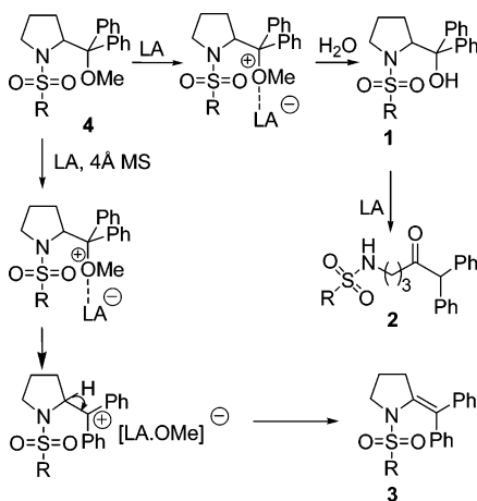
SCHEME 4. Proposed Mechanism for the Rearrangement of \alpha,\alpha -Disubstituted Methyl Ether of 5-Membered N -Tosyl Cyclic Amine 4
