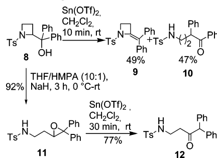
SCHEME 5. Ring Opening of the Activated Four-Membered Ring
